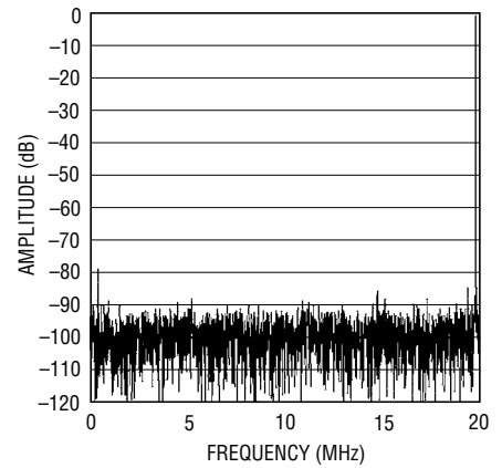
LTC2237: 8192 Point FFT, f_{IN} = 140\text{MHz} , -1\text{dB} , 2\text{V} Range, 40\text{MSPS}
