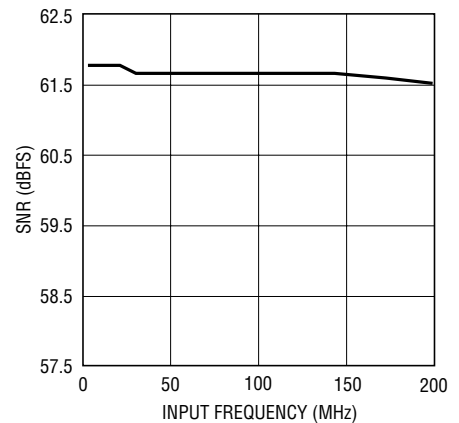
LTC2237: SNR vs Input Frequency, -1\text{dB} , 2\text{V} Range, 40\text{MSPS}
