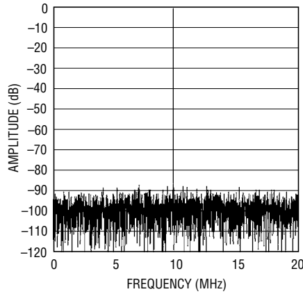
LTC2237: 8192 Point FFT, f_{IN} = 70\text{MHz} , -1\text{dB} , 2\text{V} Range, 40\text{MSPS}
