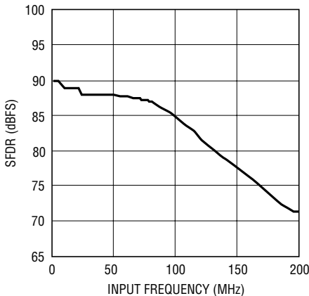
LTC2237: SFDR vs Input Frequency, -1\text{dB} , 2\text{V} Range, 40\text{MSPS}
