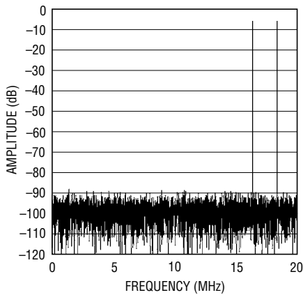
LTC2237: 8192 Point 2-Tone FFT, f_{IN} = 21.6\text{MHz} and 23.6\text{MHz} , -1\text{dB} , 2\text{V} Range, 40\text{MSPS}
