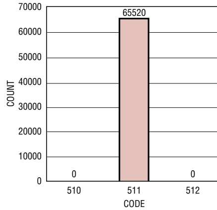
LTC2237: Grounded Input Histogram, 40\text{MSPS}
